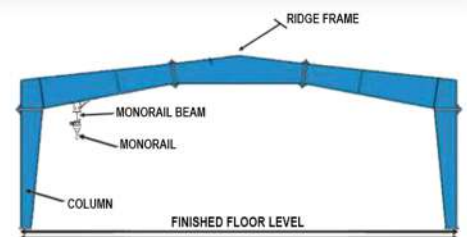
MONORAIL CRANE
