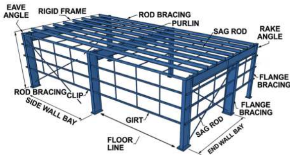
PURLINS (CONTINUOUS SUPPORT)
