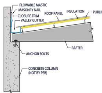
Roof System with Insulation
